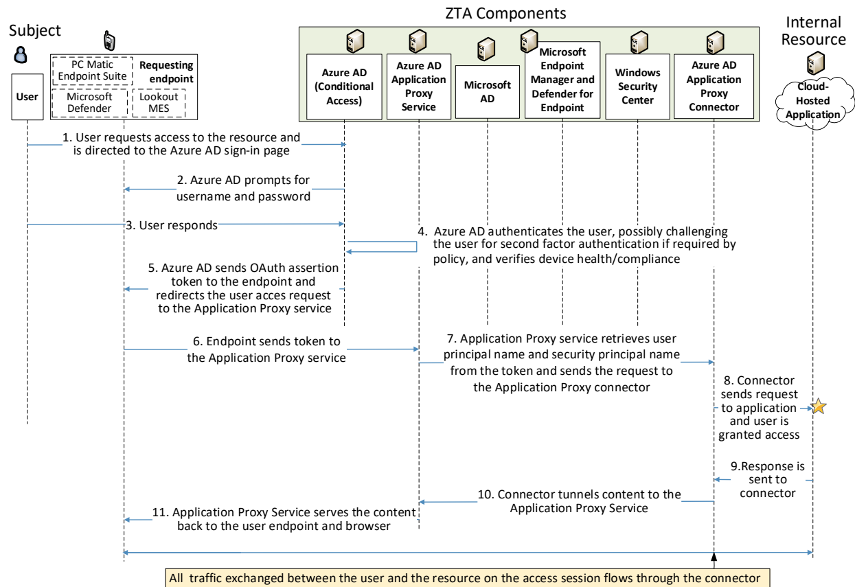
3725 Figure J-2 Use Case— E3B2 – Access to an Internal Resource is Enforced by Azure AD and Azure AD’s 3726 Application Proxy
