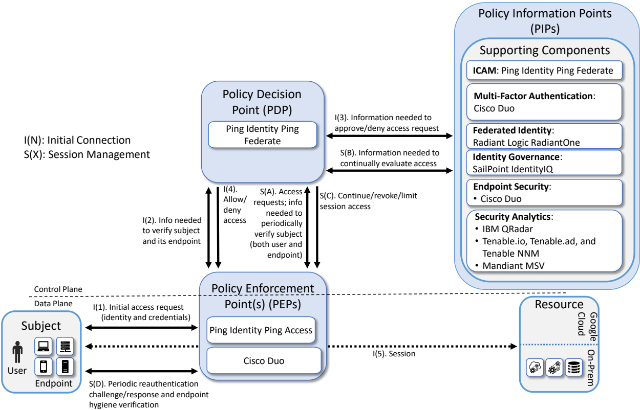
Figure E-1 Logical Architecture of E2B1
