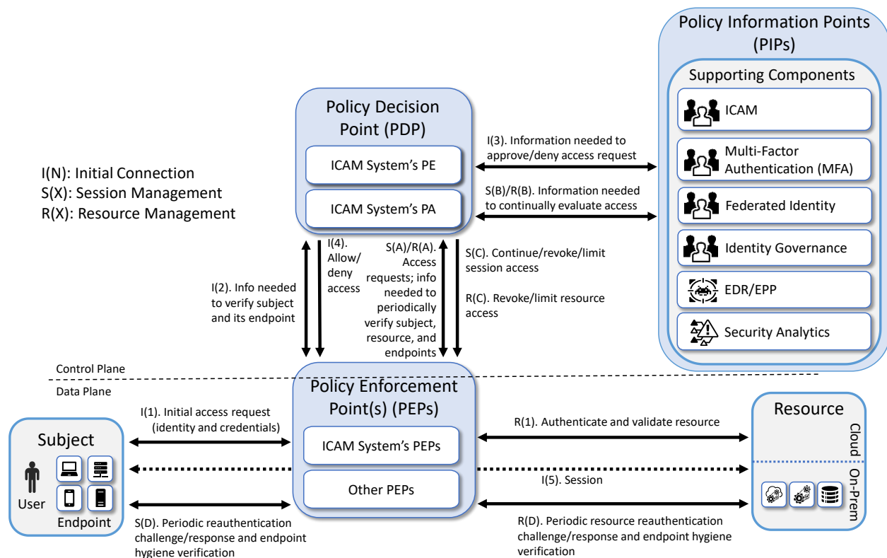
2231 Figure 4-2 EIG Crawl Phase Reference Architecture
